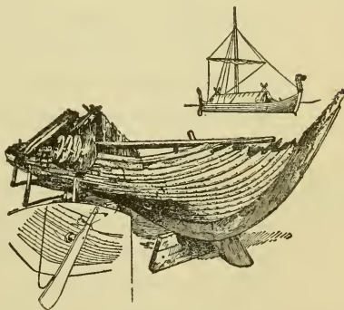
THE BOW OF THE VIKING SHIP OF GOKSTAD, SHOWING RESTORED STEERING BOARD ON THE LEFT, AND COMPLETE SHIP ABOVE
